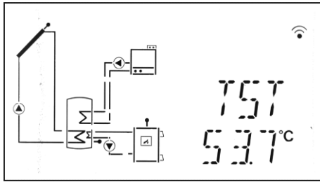
Boiler ON Solid fuel boiler (SFB ON)
