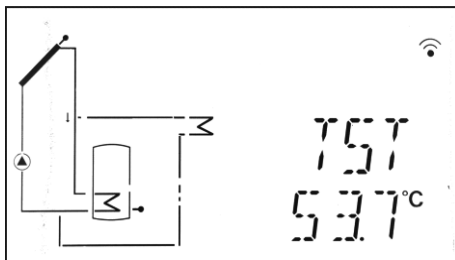
Pump logic (OTPUM ON)
